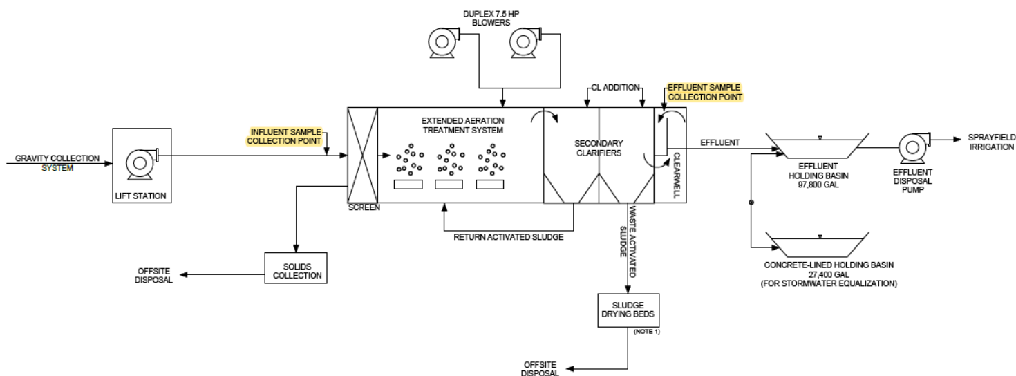
Figure 1. Process Flow Diagram with Sampling Locations
