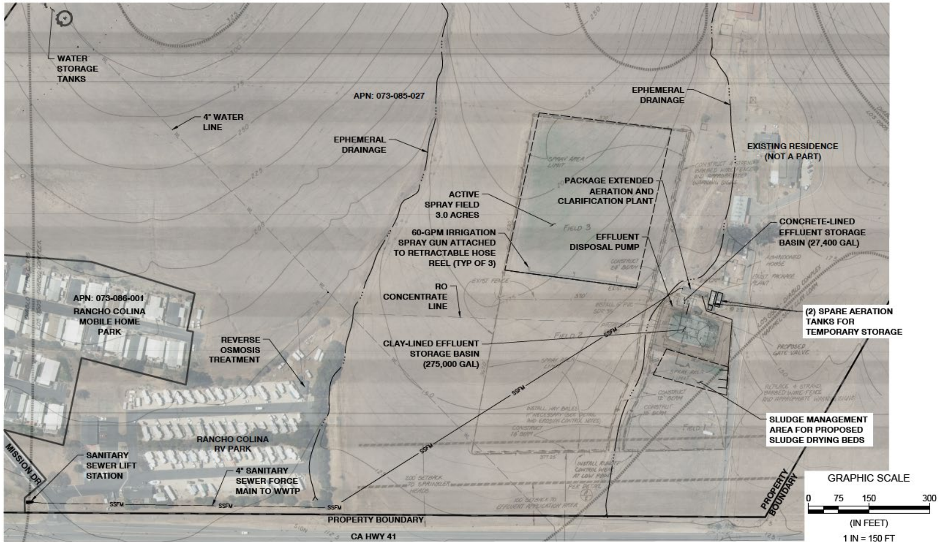
Figure 3. Site Map and Disposal Site Plan
